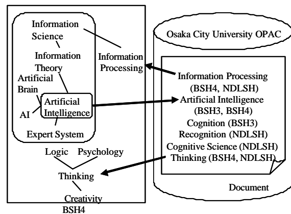
Figure 3: Overview of example 1.
