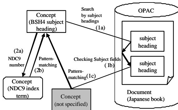
Figure 1: Framework of integrating heterogeneous terminology.
